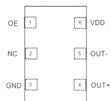
Figure 1. Pin Assignments
