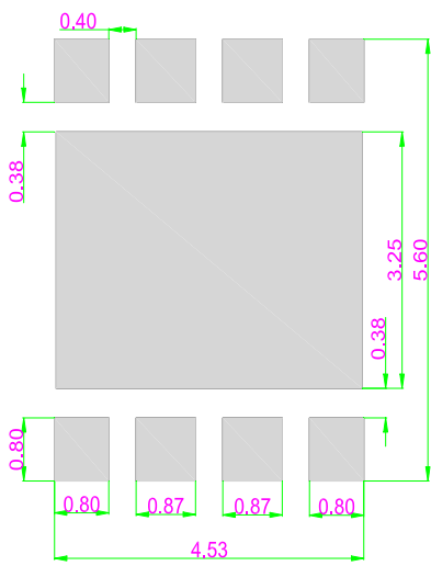
Recommended PCB Solder Pad
