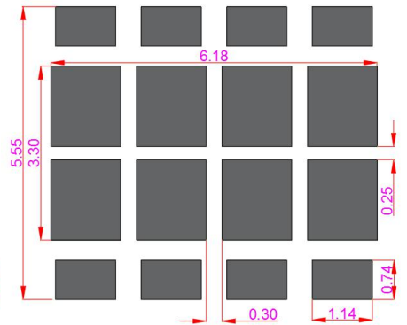
Recommended Stencil Pattern
