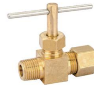
DH-N1705 Item# Description DH-N1705-1 1/4"CompX1/8"MIP DH-N1705-2 1/4"CompX1/4"MIP
