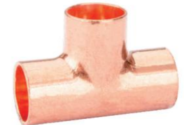
DH-O1120 Copper Tee Description Item# Description DH-O1120-1 1/4" DH-O1120-2 3/8" DH-O1120-3 1/2" DH-O1120-4 1/2" x 1/2" x 3/4" DH-O1120-5 3/4" x 1/2" x 1/2" DH-O1120-6 3/4" x 3/4" x 1/2" DH-O1120-7 3/4" x 1/2" x 3/4" DH-O1120-8 3/4" DH-O1120-9 3/4" x 3/4" x 1" DH-O1120-10 1" x 1" x 1/2" DH-O1120-11 1" x 1/2" x 1" DH-O1120-12 1" x 3/4" x 3/4" DH-O1120-13 1" x 3/4" x 1" DH-O1120-14 1" x 1" x 3/4" DH-O1120-15 1" DH-O1120-16 1-1/4" x 1" x 1" DH-O1120-17 1-1/4" x 1-1/4" x 3/4" DH-O1120-18 1-1/4" x 1-1/4" x 1" DH-O1120-19 1-1/4" DH-O1120-20 1-1/2" DH-O1120-21 1-1/2" x 1-1/2" x 1-1/4" DH-O1120-22 2" DH-O1120-23 2" x 1-1/2" DH-O1120-24 3"
