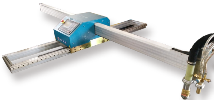
Maximum Plasma Cutting Thickness of up to 32mm(1.25in)
