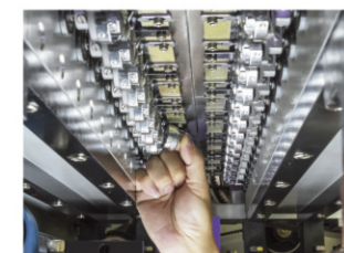
双排旋梭设计 Double row rotary shuttle design
