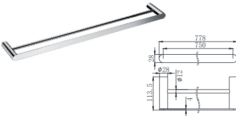
15-8804/750 Double Towel Bar Chrome
