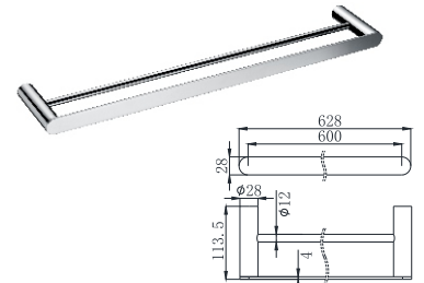
15-8804/600 Double Towel Bar Chrome
