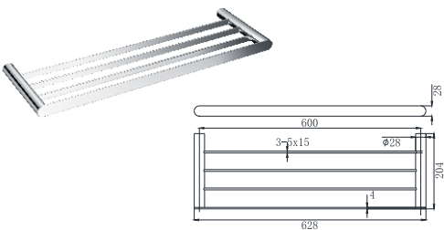
15-8808 Towel Rack Chrome
