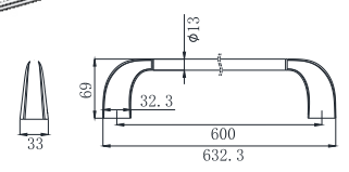
18-8908/600 Towel Bar Chrome
