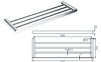
15-8807 Towel Rack Chrome
