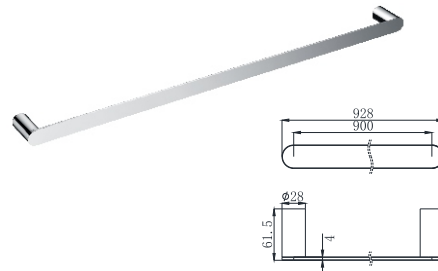
15-8803/900 Towel Bar Chrome
