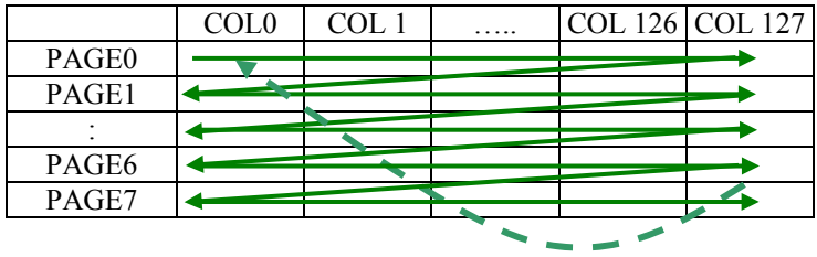
Figure 9-3 : Address Pointer Movement of Horizontal addressing mode
