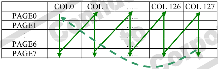
Figure 9-4 : Address Pointer Movement of Vertical addressing mode
