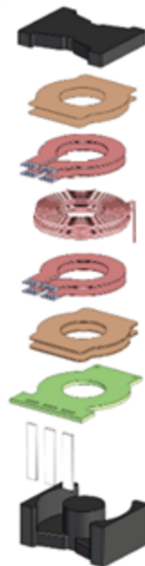
Planar Transformer
