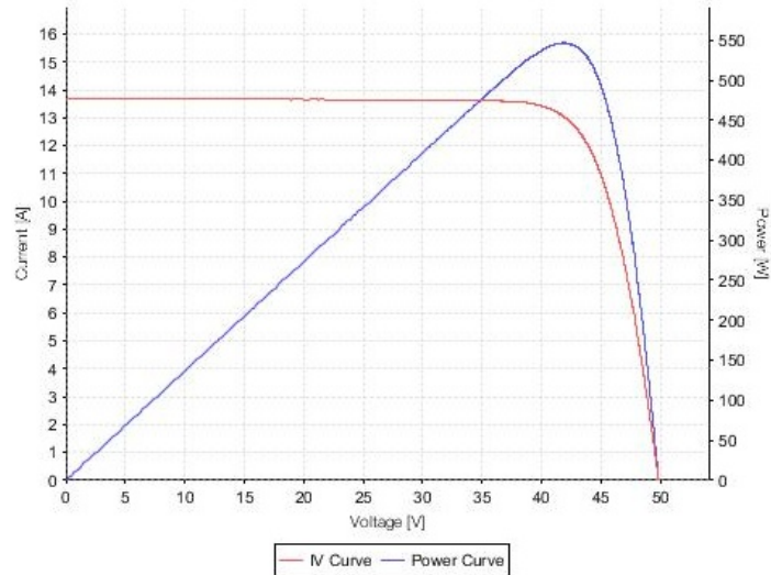
Fig. 5 IV curve of module No.1 Serial number: AS221803037900
