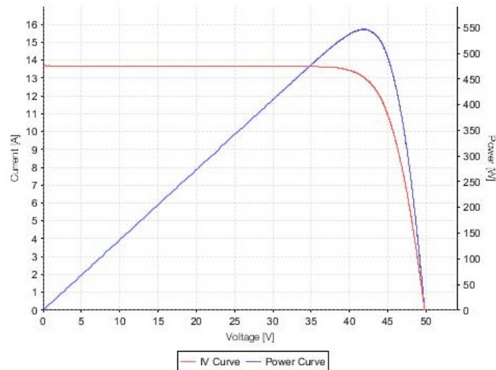
Fig. 6 IV curve of module No.2 Serial number: AS221803037883
