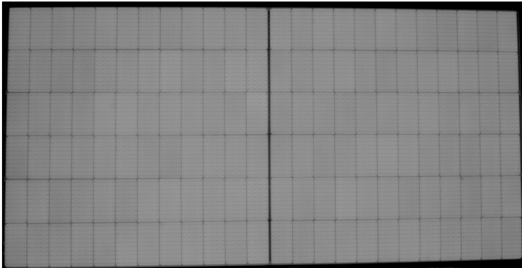
Fig. 8 EL photo of module No.2 Serial number: AS221803037883
