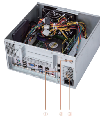
①.PCIE Slot position ②.Power SW ③.Power position
